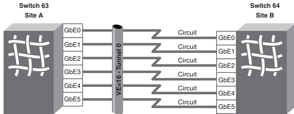
FIGURE 13 FCIP tunnel example with six circuits
